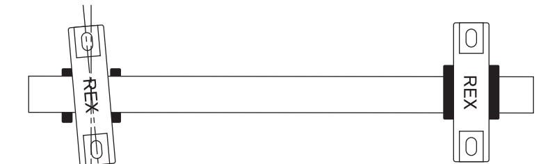
Bolts on Left Bearing are Vertically Misaligned
