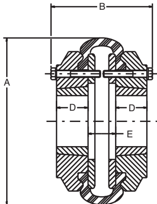
PX40 STANDARD COUPLING TYPE F TAPER-LOCK
